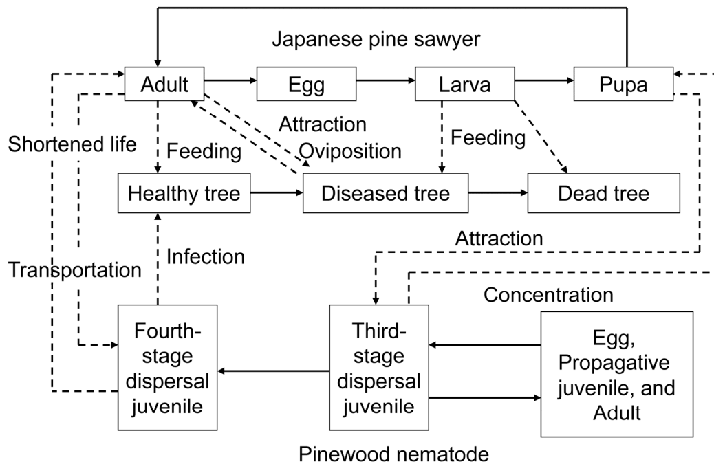
Fig. 1. Relationships between the pinewood nematode ( Bursaphelenchus xylophilus ), the Japanese pine sawyer ( Monochamus alternatus ), and trees of the genus Pinus in pine wilt disease system. Solid and broken arrows represent the change of stages or states and the action, respectively. (modified from Togashi, 1989e)
