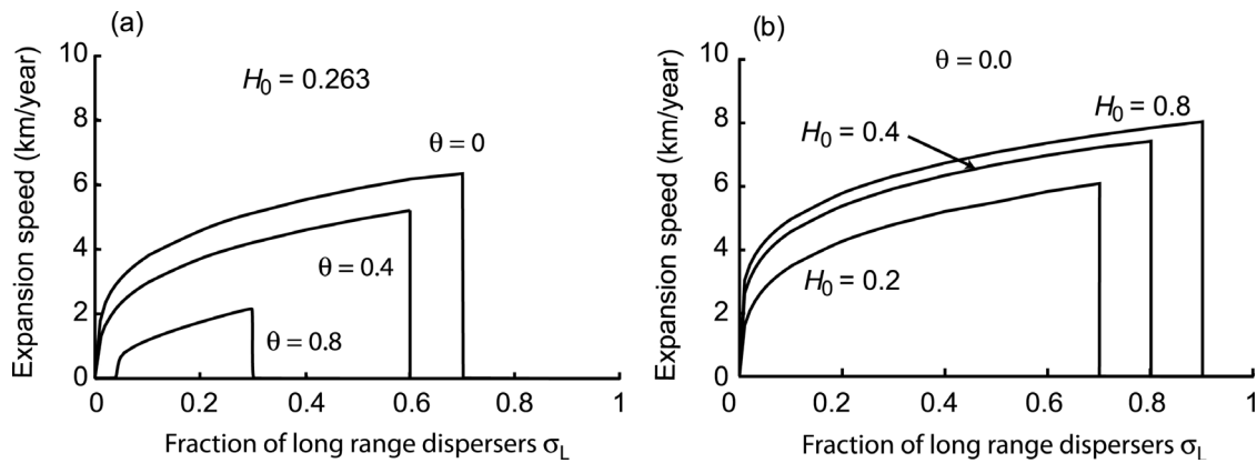
Fig. 4. Dependence of the range expansion rate of the pinewood nematode on the fraction of long-distance dispersers, \sigma_L . (a) The initial pine density is fixed as H_0 = 0.263/m^2 , while the eradication rate, \theta , is varied as indicated, (b) the eradication rate is fixed as \theta = 0 , while H_0 is varied as indicated. (after Fig. 7 of Takasu et al. , 2000)
