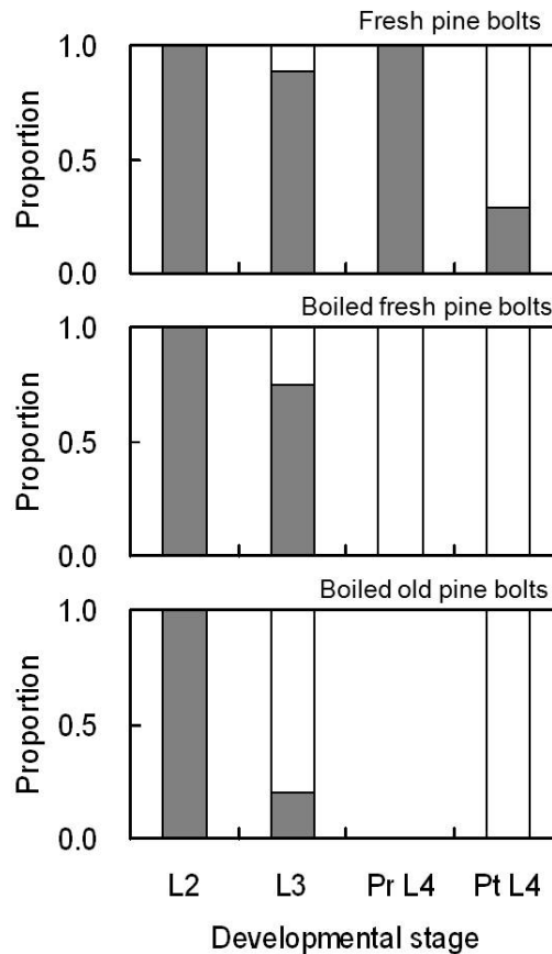
Fig. 6. Developmental responses of different instars of Monochamus alternatus endai overwintering larvae to fresh bolts and boiled fresh and old bolts of Pinus densiflora . Horizontal axis indicates the developmental stages of larvae inoculated into pine bolts; L2, L3, Pr L4, and Pt L4 for second, third, pre-diapause fourth, and diapause fourth instars, respectively. Grey and white parts of bars indicate the living diapause larvae and emerging adults in autumn. Dead insects were excluded from the calculation of proportion. (after Togashi, 1995)
