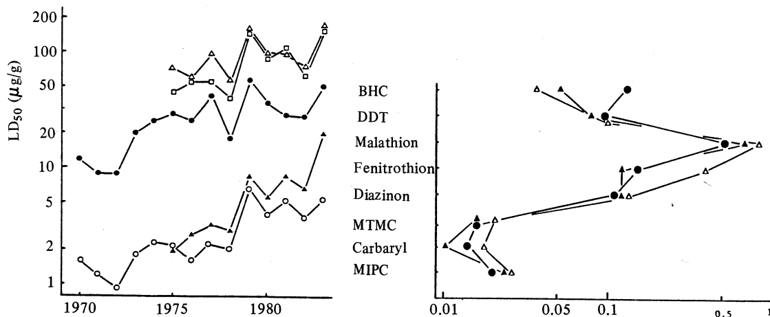
Fig. 2. Insecticide-resistance patterns of immigrant and East China Sea population of BPH (1980). △: 1st migration wave, ▲: 2nd migration wave, ●: East China Sea population.
